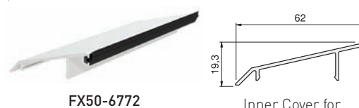
Inner Cover for 17,52 mm Glass
